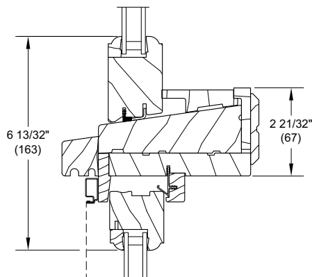
Transom mullion over WUDH
