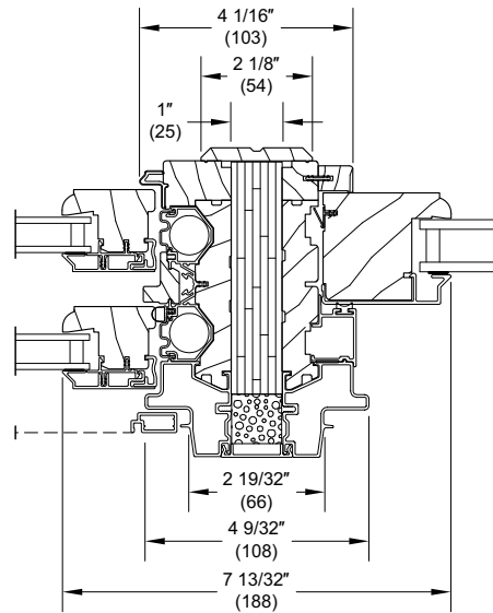
1" Solid Space Vertical Mullion Operator/Picture
