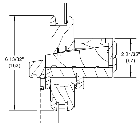
RT Transom mullion over WUDH
