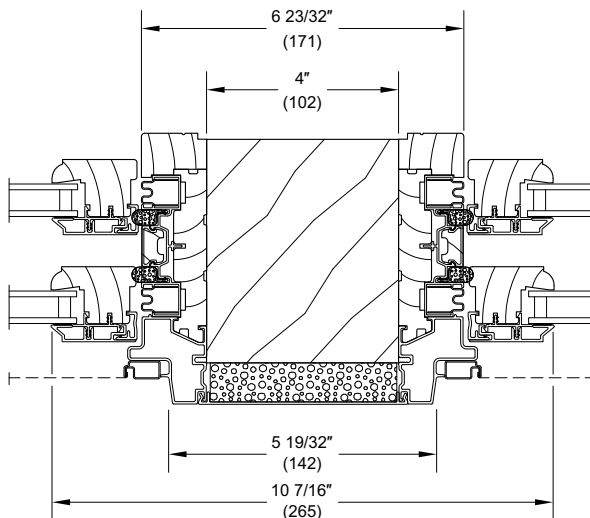
4" Space Mull
