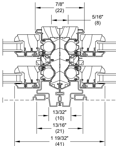
Vertical Mullion Operator/Operator
